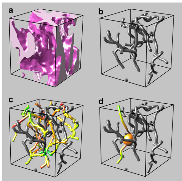
FIGURE 2 Illustration of the three-dimensional image data analysis on a small ( 5 \mu\text{m} ) 3 subset of Gel 3 (2.4 mg/ml). (a) Binary data set; all voxels with I(p) > I_c represent the collagen phase. The fiber thickness overestimates the width of collagen fibers ( 0.15 \mu\text{m} ), in particular in the vertical z direction. (b) The medial axis of the collagen domain as a one-dimensional curve representation of the fibers. (c) Medial axis of the fluid phase, i.e., the complement of the collagen fibers, as a network of widest paths through the collagen matrix. The color indicates the distance to the nearest collagen fiber, with distance increasing from red to blue. (d) A single percolating path of the fluid medial axis together with the bottleneck sphere at its point with minimal distance.
